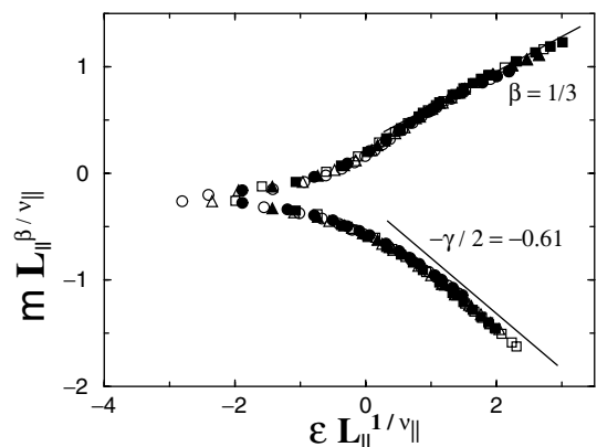
FIG. 1. Log-log plot of the order parameter rescaled by L_{\parallel}^{\beta/\nu_{\parallel}} vs \epsilon L_{\parallel}^{1/\nu_{\parallel}} , for different system sizes: (O) 45 \times 30 ; ( \Delta ) 80 \times 40 ; ( \square ) 125 \times 50 . Filled (empty) symbols stand for the RDLG (IDLG); error bars are smaller than the symbols.
