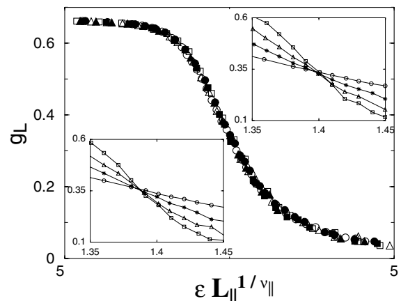
FIG. 3. Scaling plot of the fourth cumulant vs \epsilon L_{\parallel}^{1/\nu_{\parallel}} . Upper (lower) inset: fourth cumulant for the IDLG (RDLG) vs T/T_0 . Symbols are as in Fig. 1.
