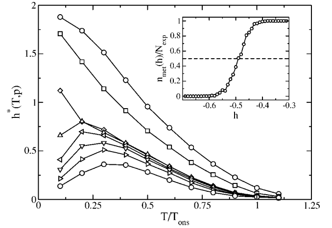
FIG. 4. Monte Carlo results for h^*(T, p) as a function of T for L=53 and, from top to bottom, p=0, 0.01, 0.03, 0.0305, 0.0320, 0.0350, 0.04, and 0.05 . Notice the change of asymptotic behavior in the low temperature limit for p \in (0.03, 0.0305) . Inset: The probability of the metastable state, as defined in the main text, as a function of h < 0 for L=53, T=0.7T_c(0), and p=0 . Data here correspond to an average over 500 independent demagnetization experiments for each value of h . Error bars are smaller than the symbol sizes.
