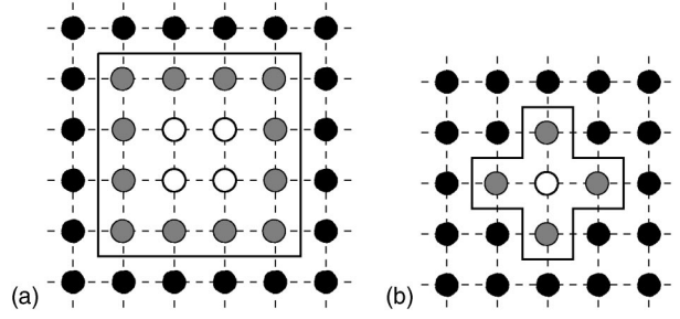
FIG. 1. Two examples of spin domains, each following from a different lattice partition P(\Lambda) ; see the main text. The spins that do not belong to the domain are in black, surface spins are gray, and the spins forming the domain interior are empty.
