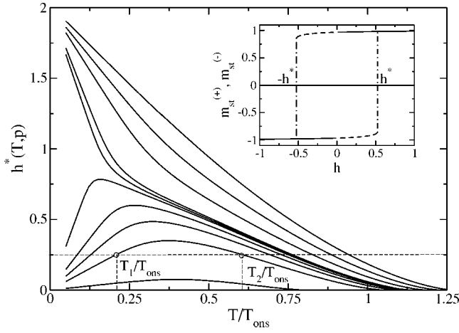
FIG. 3. h^*(T, p) , as a function of T for, from top to bottom, p = 0, 0.01, 0.02, 0.03, 0.031, 0.032, 0.035, 0.04, 0.05 , and 0.1 . The qualitative change of behavior in the low temperature region occurs for p \in (0.031, 0.032) . Inset: The two locally-stable steady magnetization branches as a function of h for T=0.7T_c(0) and p=0.005 . The solid (dashed) line represents stable (metastable) states. The dotted-dashed line signals the discontinuous transition, at h = h^*(T, p) , where metastable states disappear.
