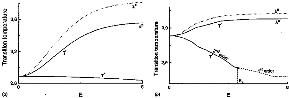
Figure 4. The field dependence of the transition temperatures T' and T^* , for \rho = \frac{1}{2} , and for (a) the Kawasaki rate, \phi(X) = 1/(1 + e^X) , and (b) the Metropolis rate, \phi(X) = \min\{1, e^{-X}\} . The latter induces the existence of a non-equilibrium tricritical point at E_c separating second- from first-order phase transitions. The function T'(E) for the ordinary, two-dimensional DLG obtained within the same approximation is also shown (curves labelled \lambda^E ).
